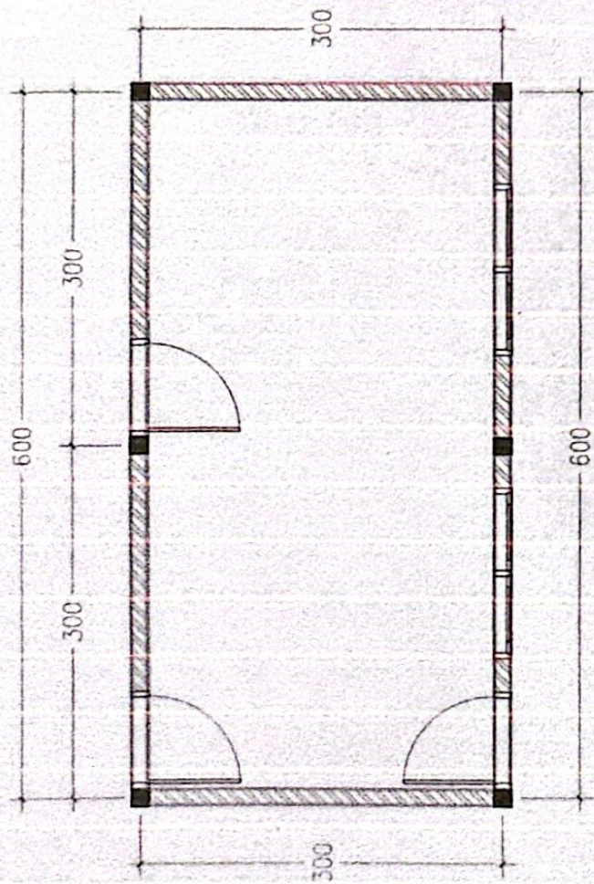
DENAH EXISTING RUANG CAMAT Skala 1 : 50
